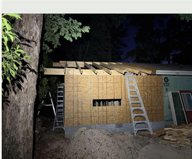
Wall framing and sheathing
