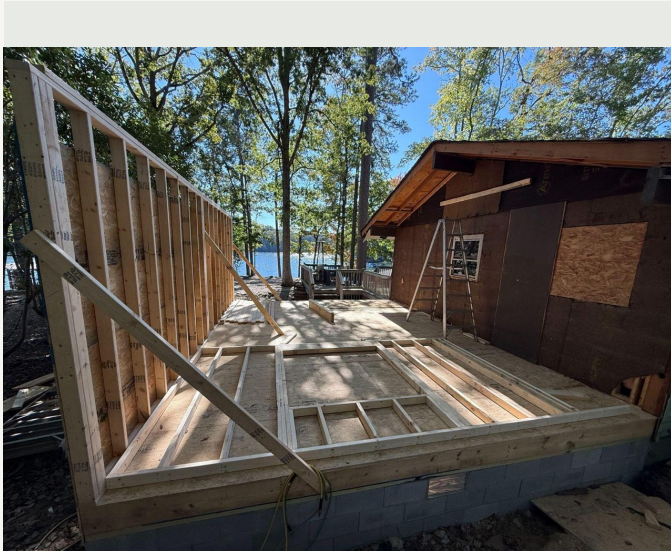
Floor framing
